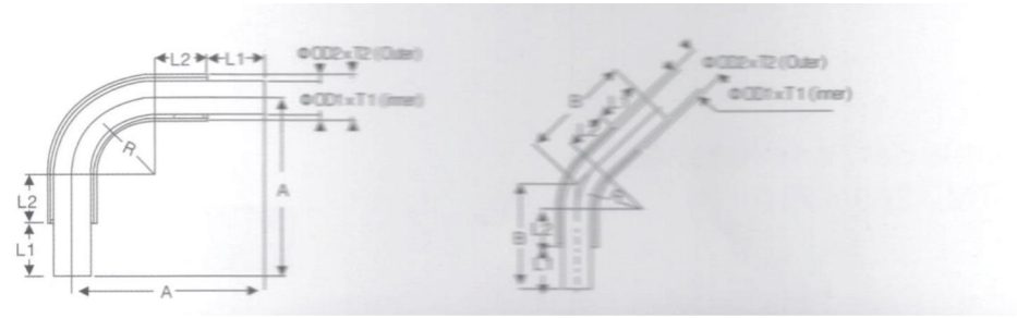
Double Set Elbow 双套弯头 ASTM A269/A270
